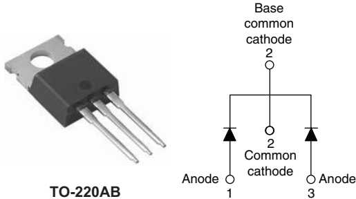
TO-220AB
